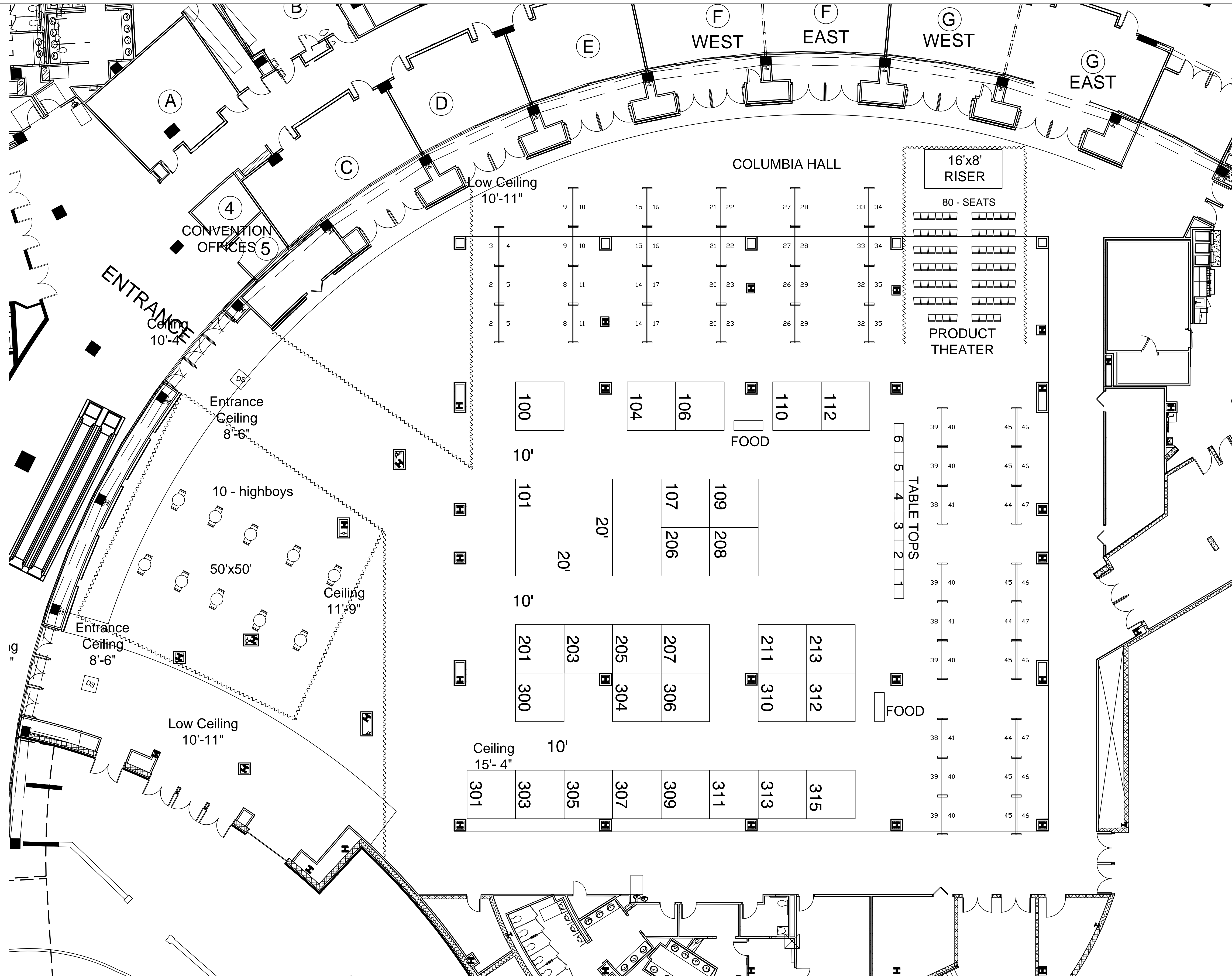
PLAN VIEW: COLUMBIA HALL SCALE: 3/32"=1'
